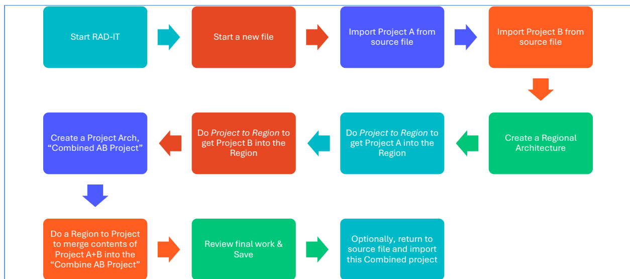
Figure 1. Flow Diagram to Merge 2 Project Architectures
